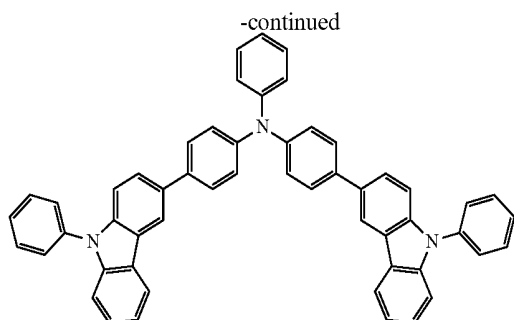
Comparative Compound C1 Comparative Compound C2 Comparative Compound C3.
